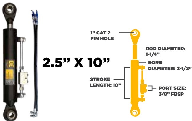
21.5 - 31.5" CATEGORY 2 HYDRAULIC TOP LINK KIT 46.225.010
