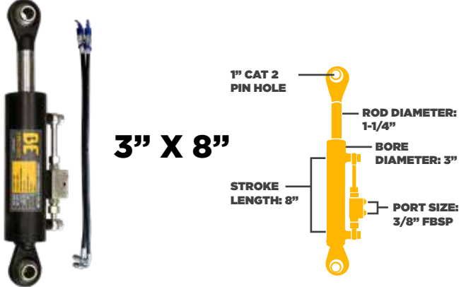
22 - 30" CATEGORY 2 HYDRAULIC TOP LINK KIT 46.230.008
