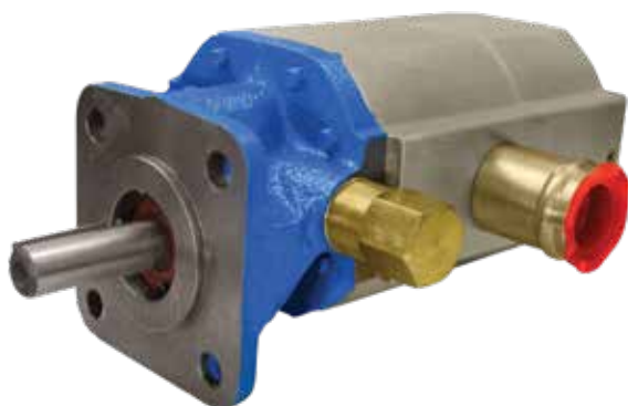
11 GPM HI/LO HYDRAULIC PUMP 2 STAGE GEAR PUMP, 1/2" SHAFT CW, 11 GPM, NOMINAL FLOW, 3000 PSI 46.333.008
