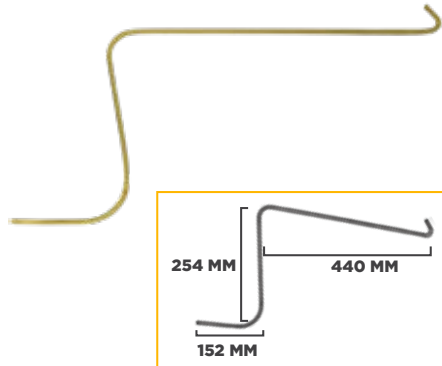
JD RAKE TINE OEM TP257SE 45.000.257
