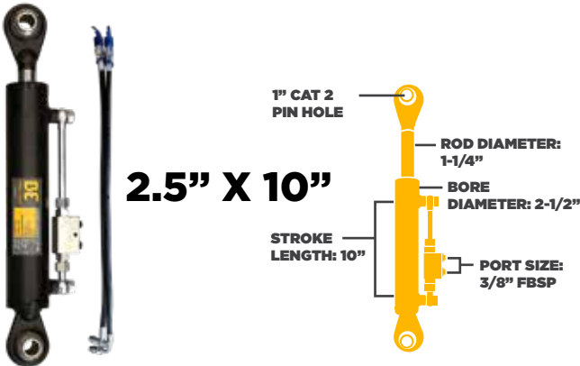
21.5 - 31.5" CATEGORY 2 HYDRAULIC TOP LINK KIT 46.225.010
