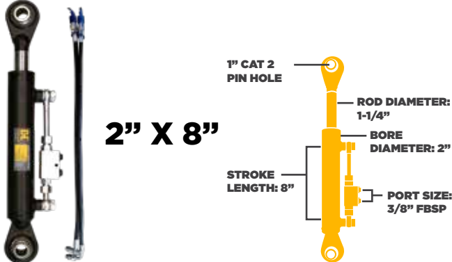
22 - 30" CATEGORY 2 HYDRAULIC TOP LINK KIT 46.230.008
