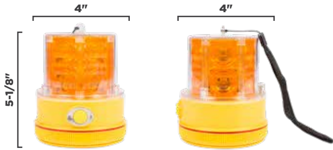
HOUSING WITHOUT HARDWARE
