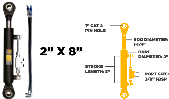
22 - 30" CATEGORY 2 HYDRAULIC TOP LINK KIT 46.230.008
