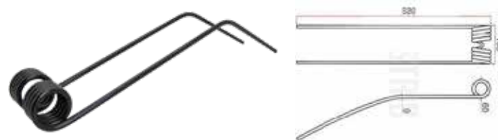
DA ROS GR TINE DA ROS, MODELS GR300/330/380/410 OEM 6900220 45.000.220
